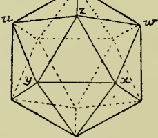
V. Icosa-hedron
